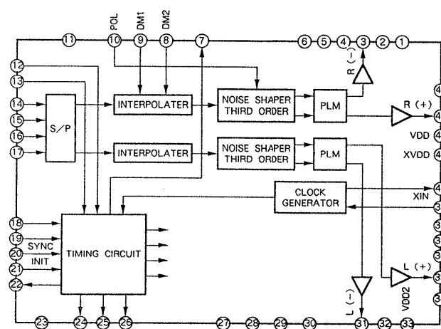
IC308 CXD2552Q
