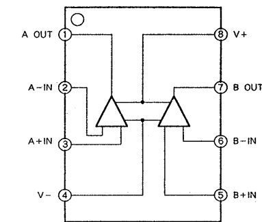
IC104 etc. NJM5532D-D
