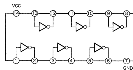
IC507 74HC05
