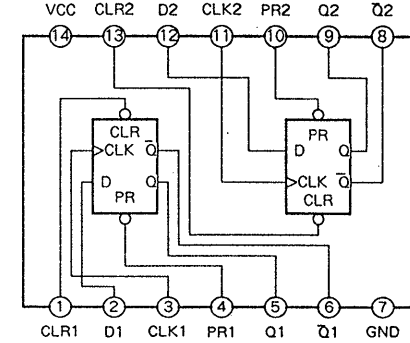
IC317 74HC74/AC74
