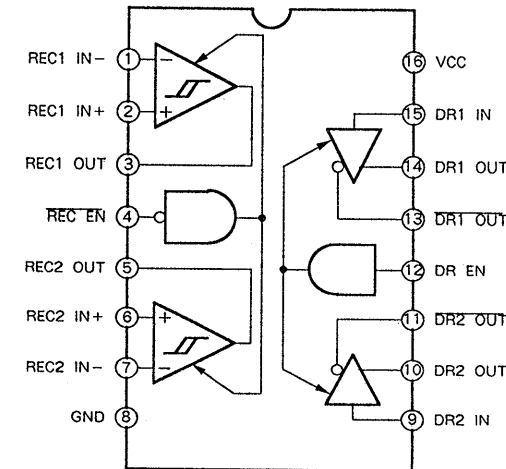
IC509 MC34050P
