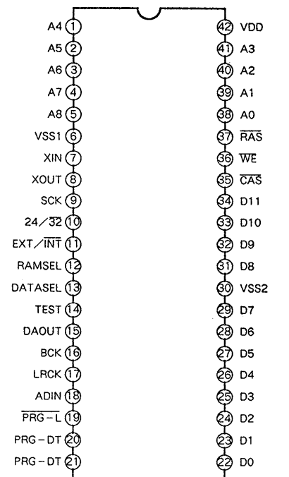
IC502 CXD8162P
