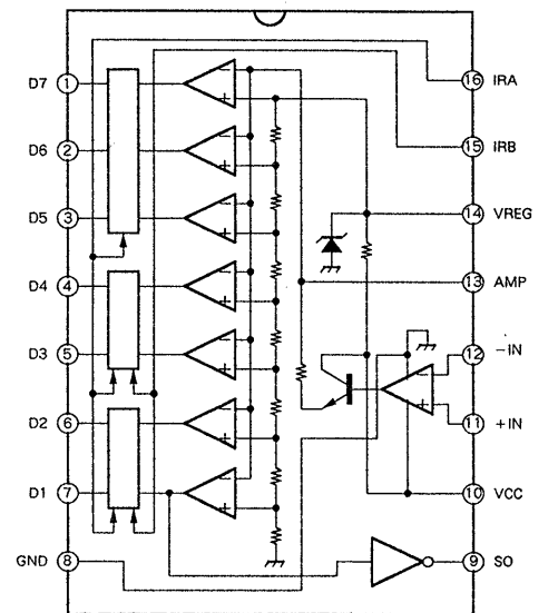
IC401, 451 IR2E02
