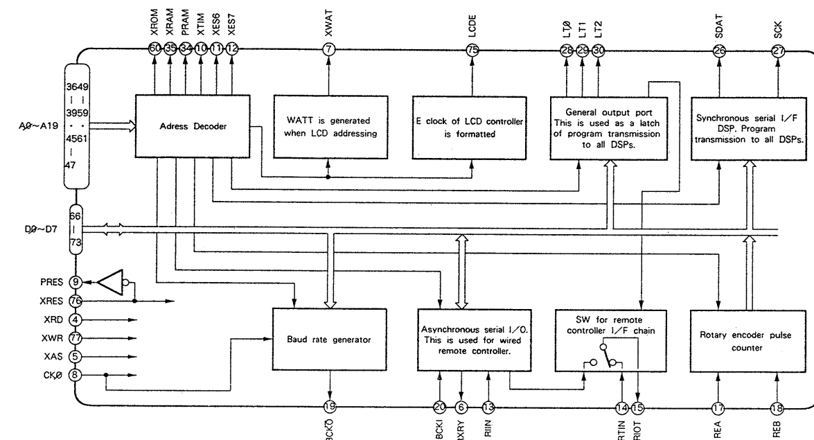
IC510 CXD2903Q
