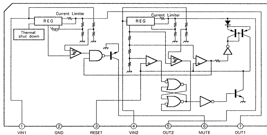
IC306 LA5665
