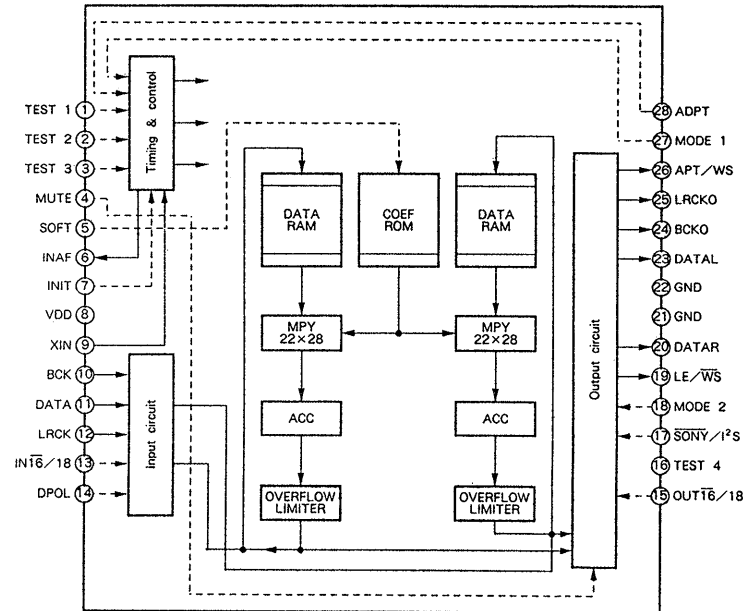
IC305 CXD1144BP
