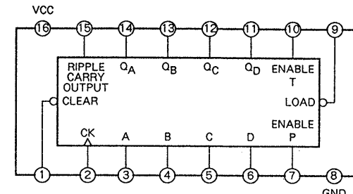
IC315, 316 74HC161
