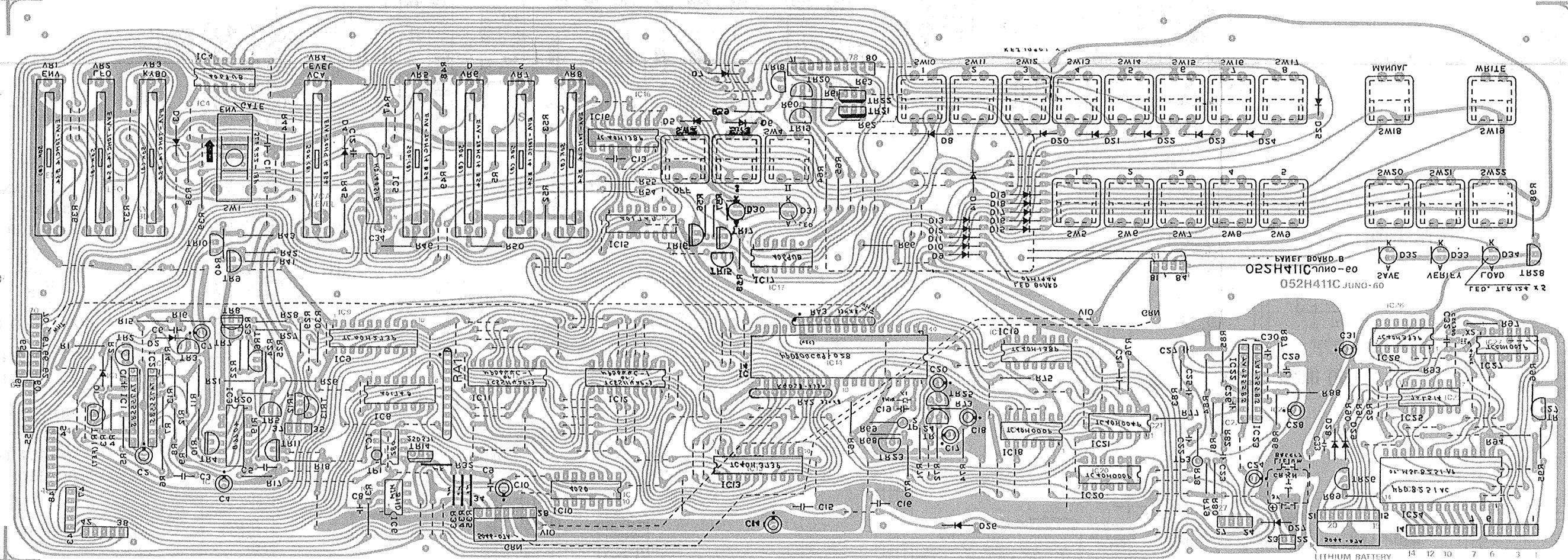
OPH188C (149H188C) (pcb 052H411C)
