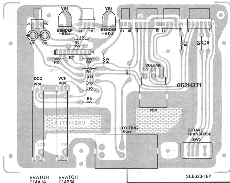
View from component side
