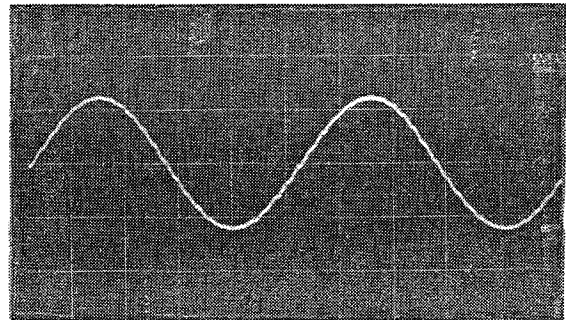
U72 pin 7 (output of output deemphasis) 2 V/DIV., 0.2 ms/DIV. 1 kHz input
